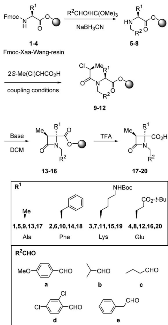
Scheme 1. Solid-phase synthetic approach to \beta -lactams 17–20 and diversity incorporated at R 1 and R 2 positions.
