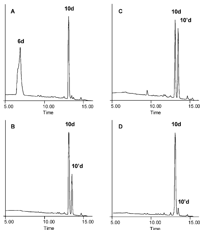
Figure 1. Optimization of the coupling procedure to intermediate 10d . A : 2( S )-chloropropionic acid/PyBrop/DIEA/THF (twice). B : 2( R,S )-chloropropionyl chloride/propylene oxide/THF. C : 2( S )-chloropropionic acid/ \text{Cl}_3\text{CCN}/\text{PPh}_3/\text{DIEA}/\text{THF} . D : 2( S )-chloropropionic acid/ \text{Cl}_3\text{CCN}/\text{PPh}_3/\text{propylene oxide}/\text{THF} .
